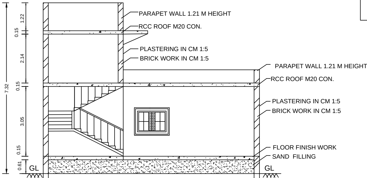
SECTION
