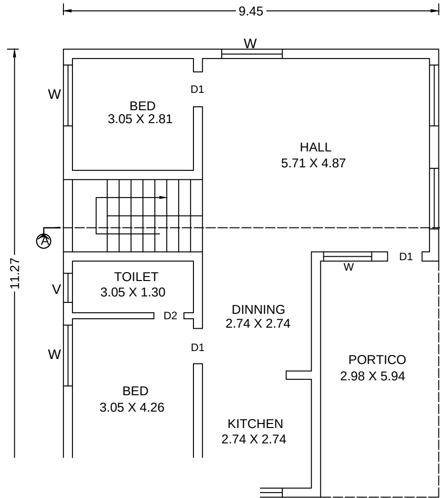
FLOOR PLAN
