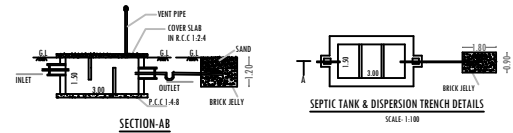
SECTION-AB
