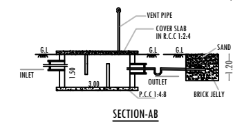
SECTION-AB
