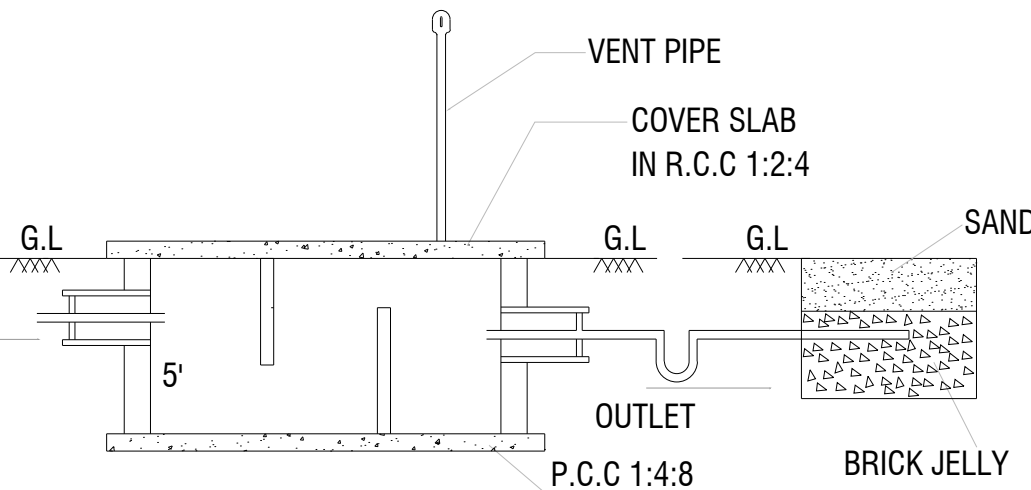
SECTION-AB
