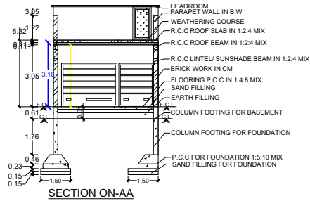
SECTION ON-AA
