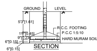
SECTION
