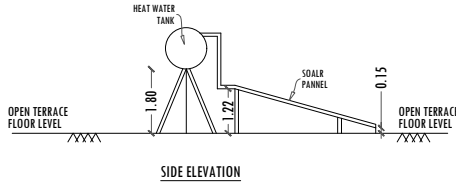
SIDE ELEVATION
