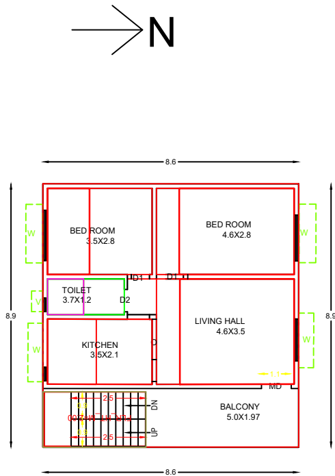
PRO.FIRTS FLOOR PLAN
