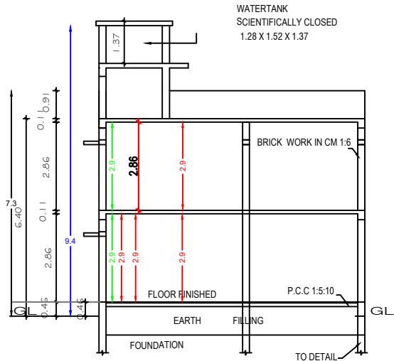
SECTION "A-B"
