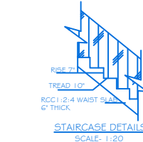
STAIRCASE DETAILS
