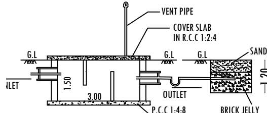
SECTION-AB
