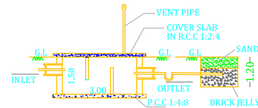
SECTION-AB
