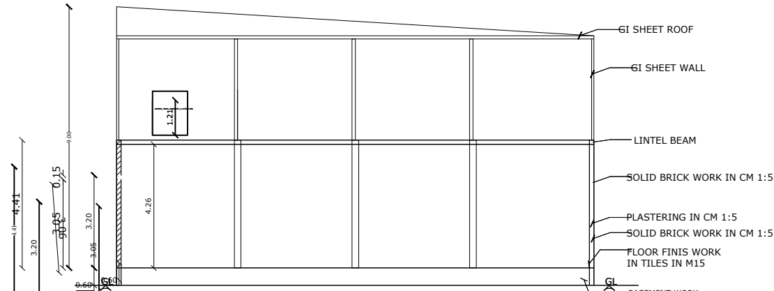
SECTION
