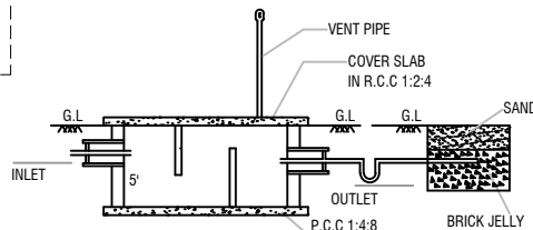
SECTION-AB
