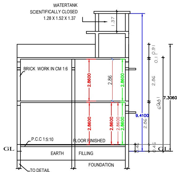
SECTION "A-B"
