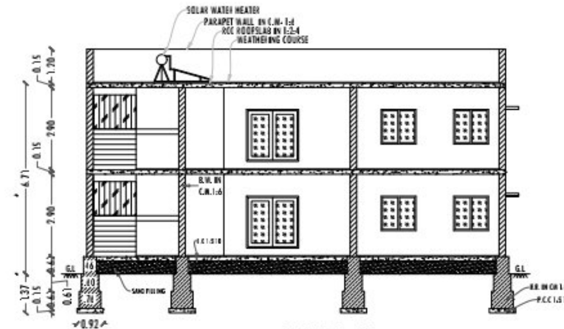
SECTION -AA
