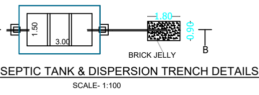
SECTION-AB
