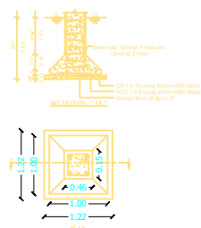
STAIRCASE DETAILS SCALE- 1:20
