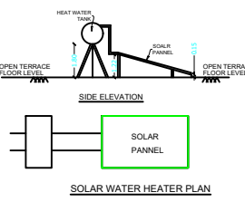
SOLAR WATER HEATER PLAN
