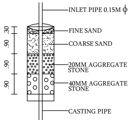
RAIN WATER HVESTING SYSTEM
