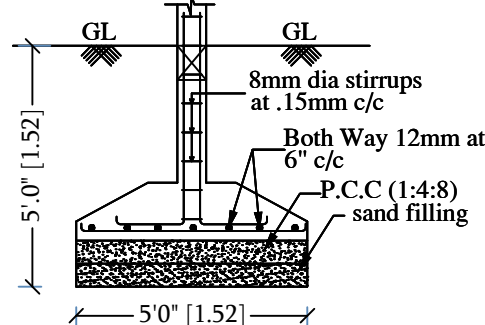
TYPICAL SECTION OF FOOTING
