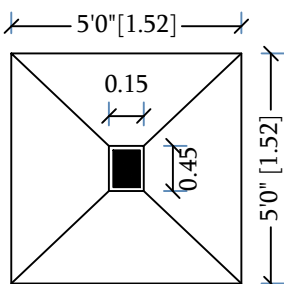
PLAN OF FOUNDATION
