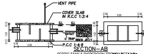
SECTION-AB SEPTIC TANK & DISPERSION TRENCH SCALE:1:100
