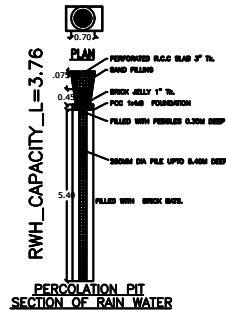
PERCOLATION PIT SECTION OF RAIN WATER
