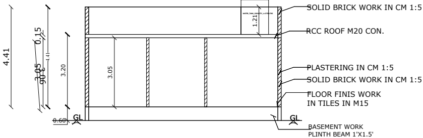
SECTION
