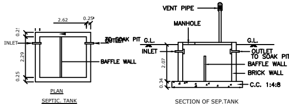
PLAN SEPTIC TANK
