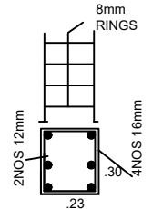
COLUMN DETAILS (NOT TO SCALE)
