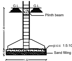
FOUNDATION DETAILS
