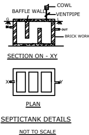
SEPTICTANK DETAILS
