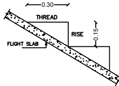
STAIRCASE DETAILS (NOT TO SCALE)
