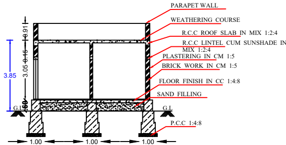
SECTION ON-"AB"
