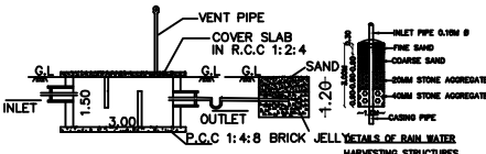
SECTION-AB
