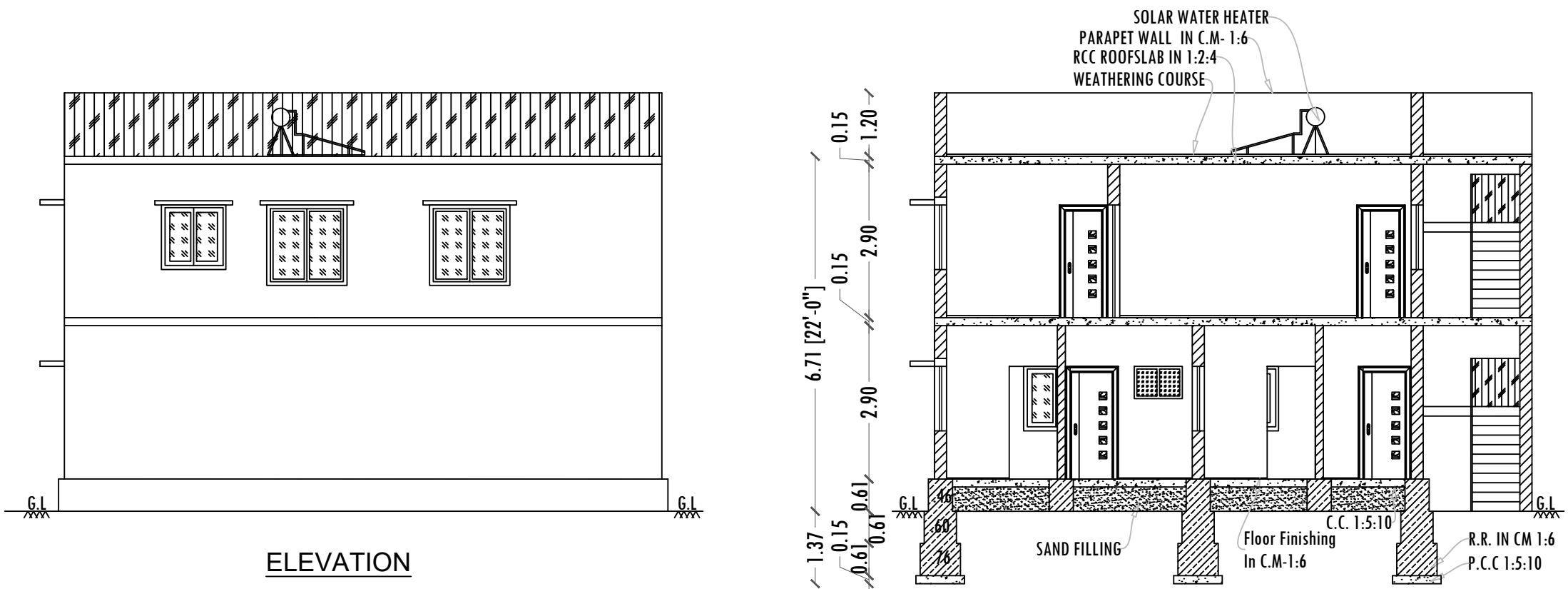
SECTION-AA
