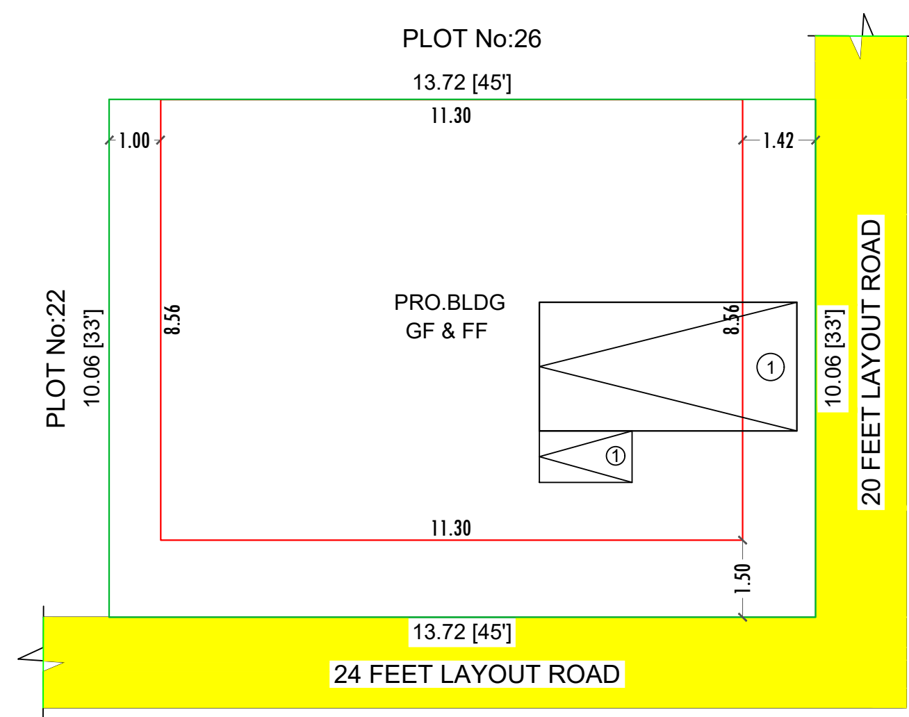
SITE PLAN
