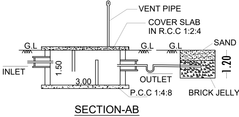
SECTION-AB
