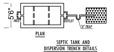
SEPTIC TANK AND DISPERSION TRENCH DETAILS
