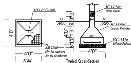
FOOTING DETAILS
