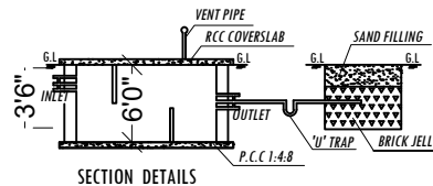
SECTION DETAILS
