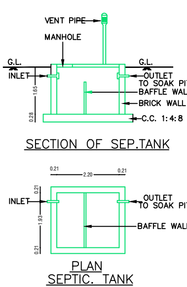
PLAN SEPTIC. TANK
