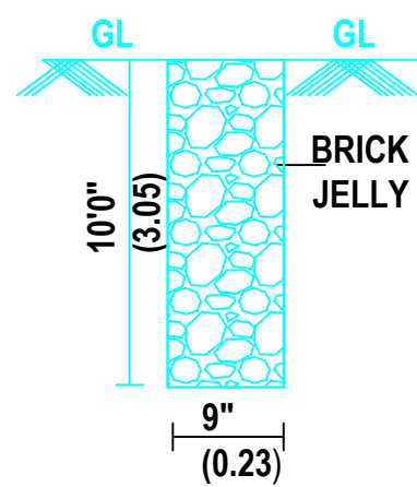
PERCULATION PIT
