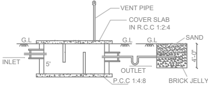
SECTION-AB
