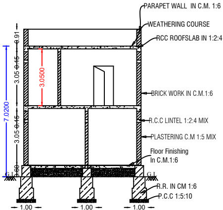
SECTION ON-'AB'
