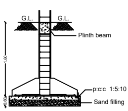
FOUNDATION DETAILS
