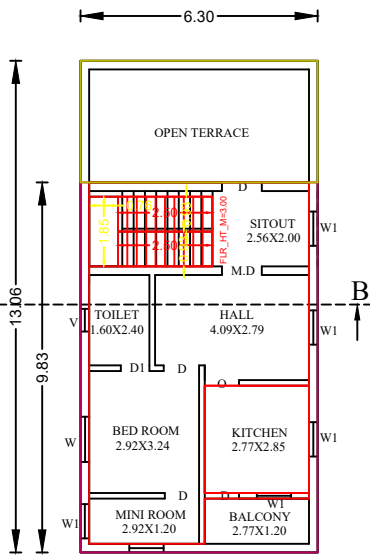
PROPOSED FRIST FLOOR PLAN
