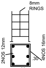
COLUMN DETAILS (NOT TO SCALE)
