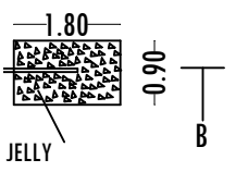
SEPTIC TANK & DISPERSTION TRENCH DETAILS SCALE: 1:100
