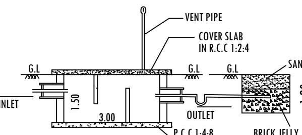
SECTION-AB
