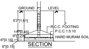
FOUNDATION DETAILS
