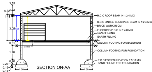
SECTION ON-AA
