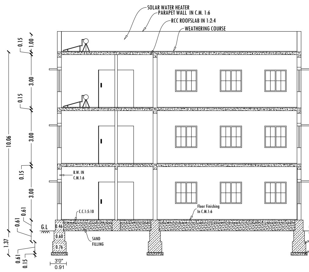
SECTION -AA
