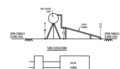
SOLAR WATER HEATER PLAN
