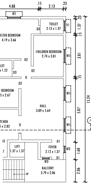
FIRST, SECOND & THIRD FLOOR PLAN
