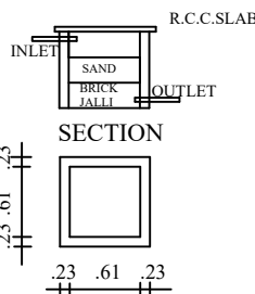
PLAN OF RAIN WATER HARVESTING PIT [SIZE: 2' X2' X 3']
