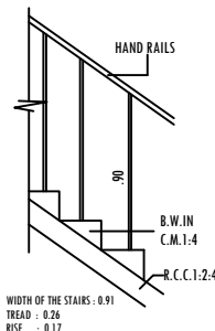
STAIRCASE DETAIL
