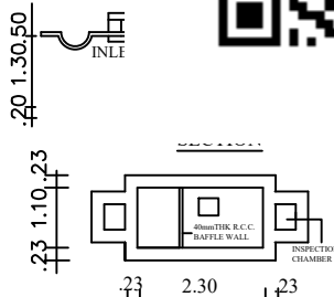
PLAN OF SEPTIC TANK
