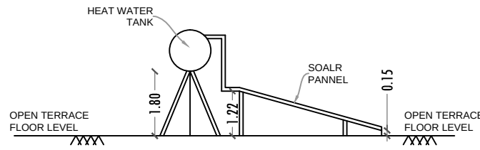
SIDE ELEVATION
