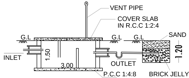
SECTION-AB
