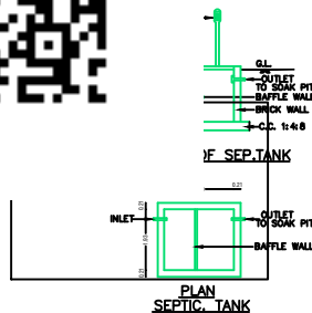
PLAN SEPTIC TANK
