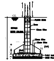
FOUNDATION DETAILS
