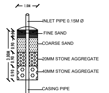
DETAILS OF RAIN WATER HARVESTING SYSTEM (NOT TO SCALE)
