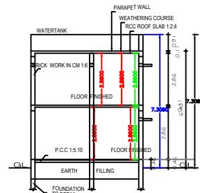
SECTION "A-B"
