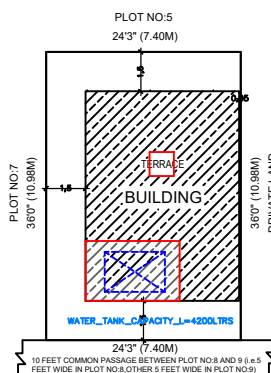
SITE PLAN
