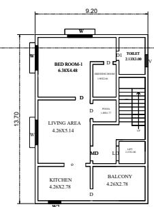
SECOND FLOOR PLAN FSI Build area-1360.56sqft/126.4sqm
