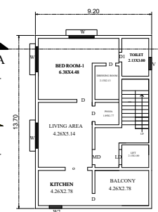
FIRST FLOOR PLAN FSI Build area-1360.56sqft/126.4sqm
