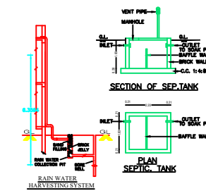
KEY PLAN SCALE : NTS.
