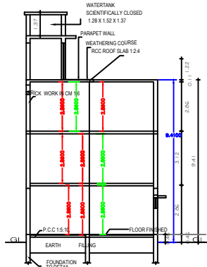
SECTION "A-B"
