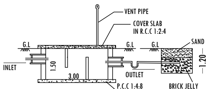
SECTION-AB
