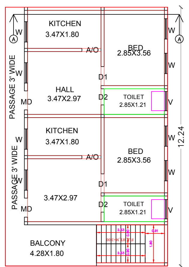
LAYOUT PLAN NOT TO SCALE
