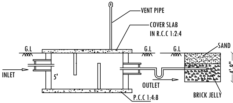
SECTION-AB
