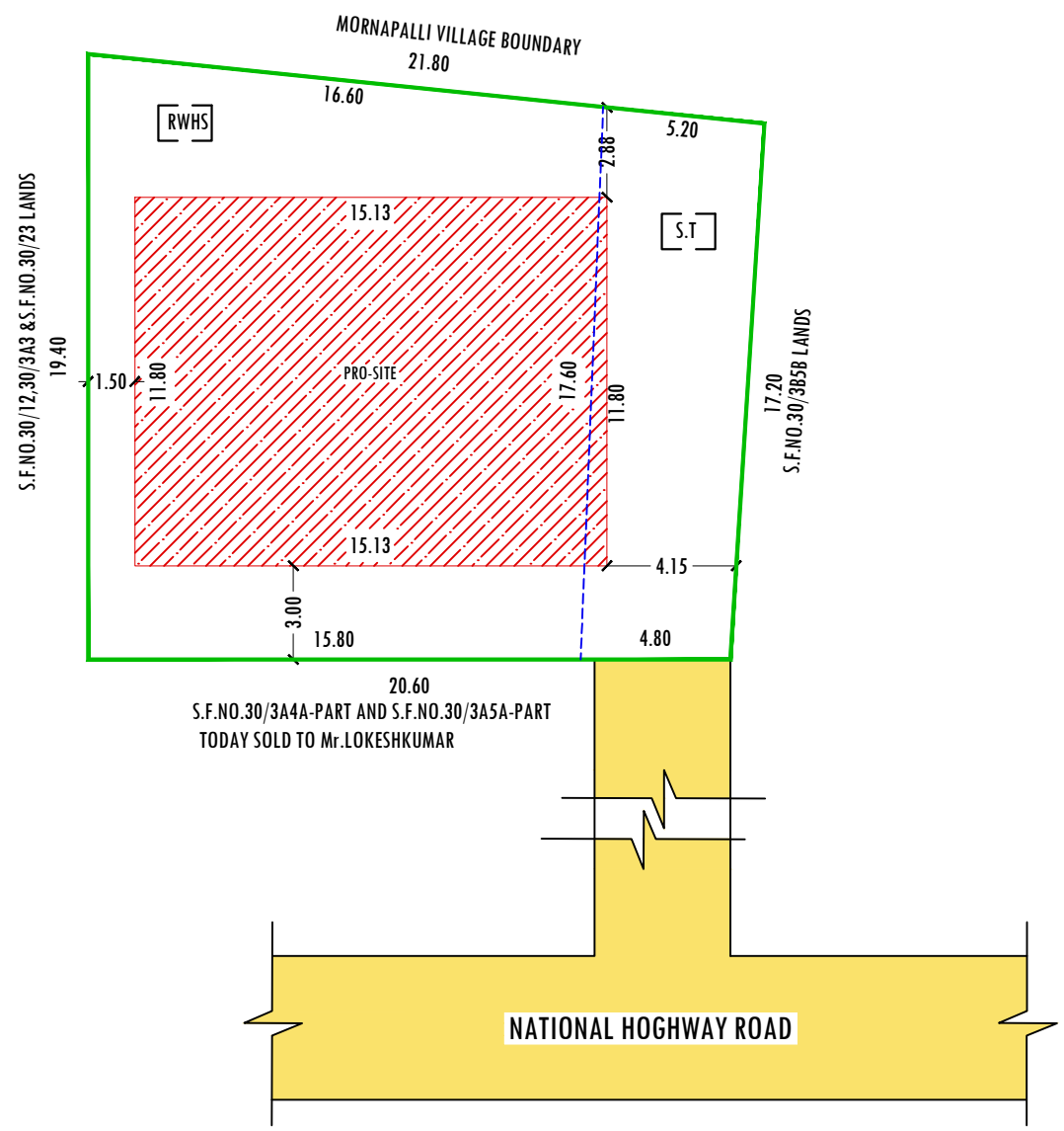
SITE PLAN
