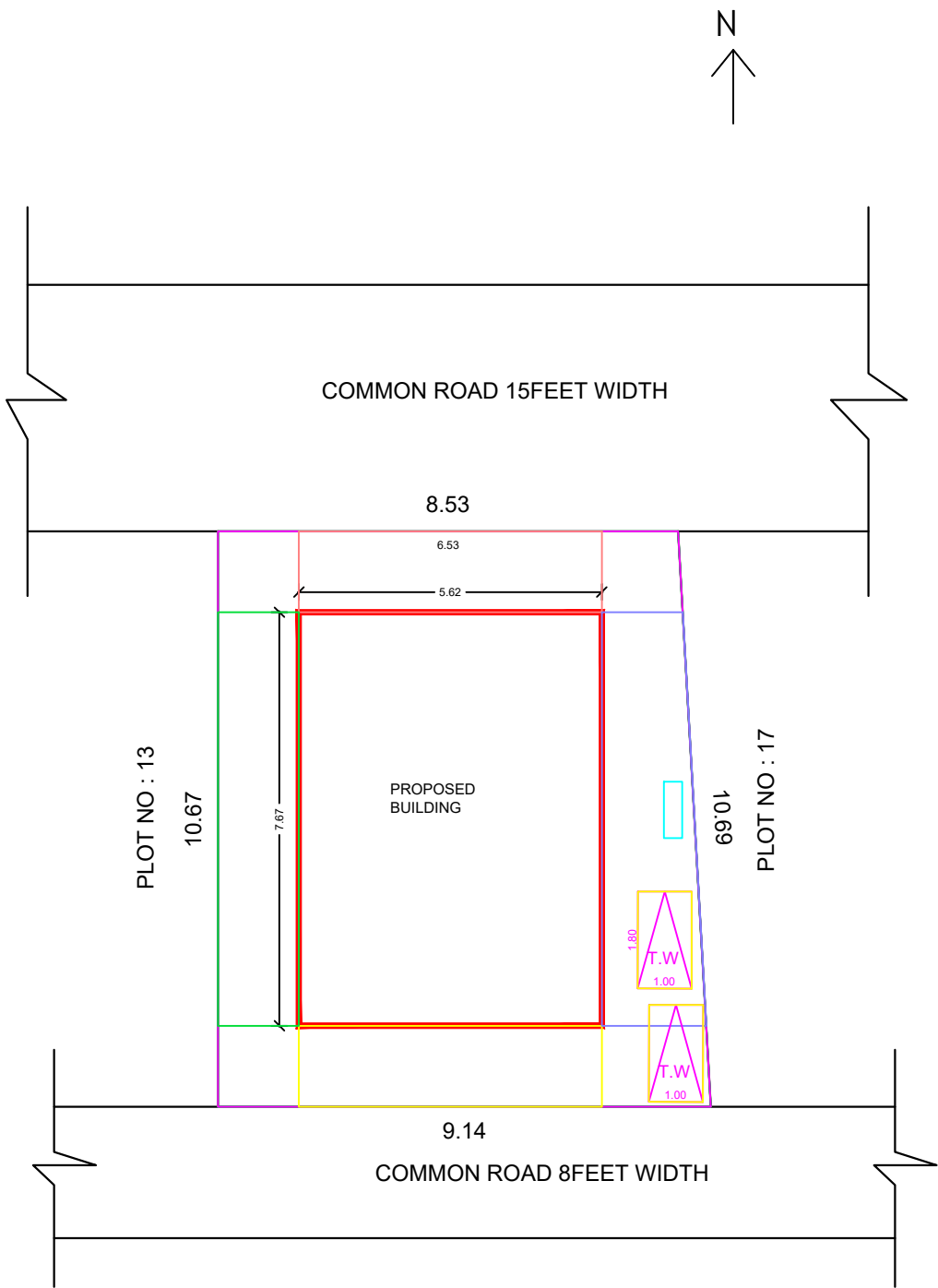
SITE PLAN
