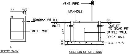
SEPTIC TANK
