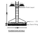
FOUNDATION DETAILS
