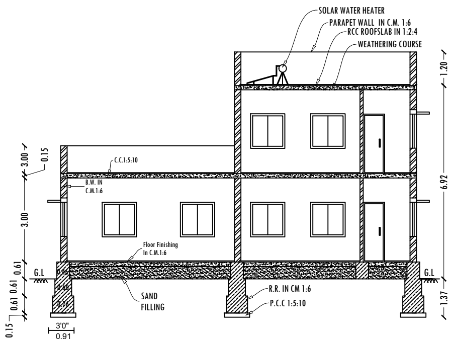
SECTION -AA
