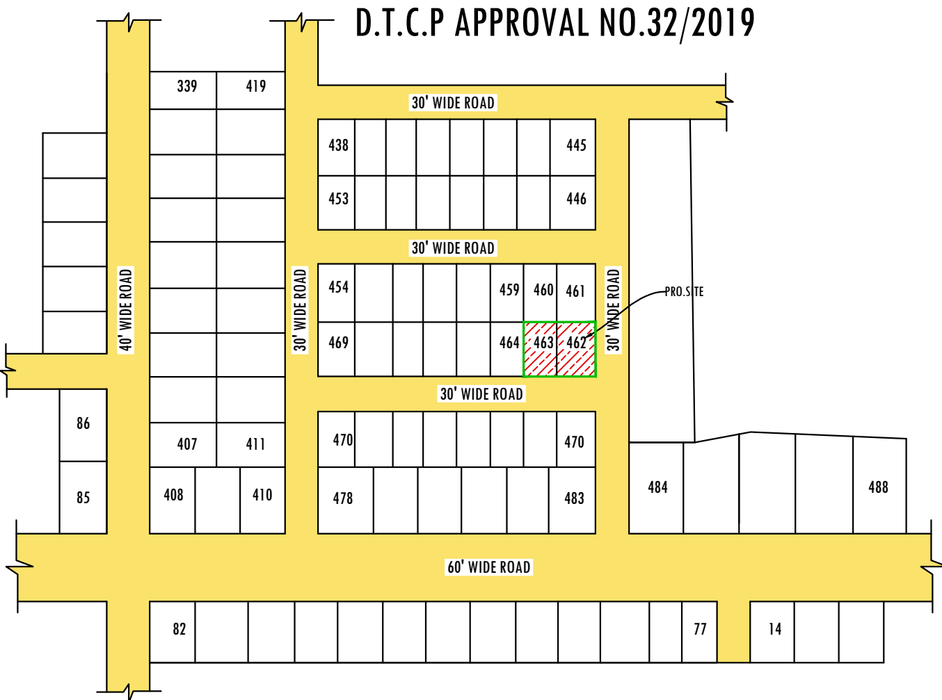
LOCATION PLAN
