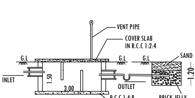
SECTION-AB
