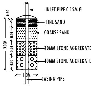
DETAILS OF RAIN WATER
