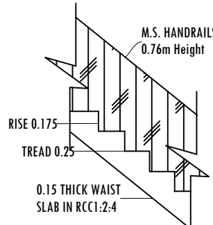
STAIRCASE DETAILS
