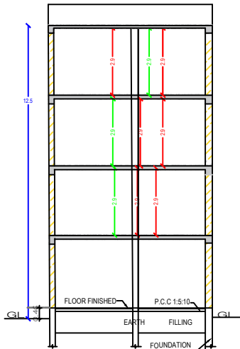
SECTION "A-B"
