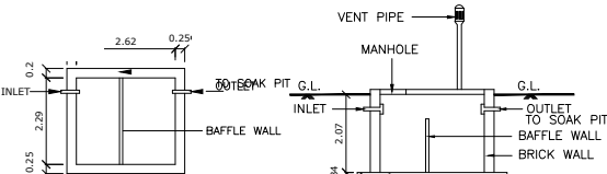
SECTION OF SEP.TANK
