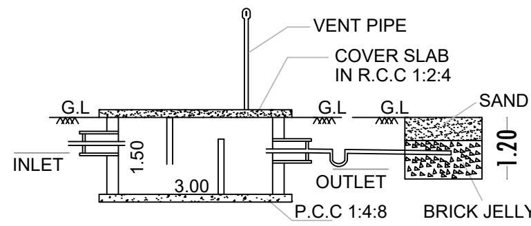
SECTION-AB
