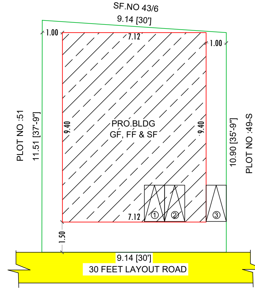
SITE PLAN
