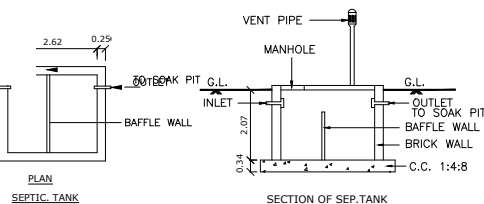
SECTION OF SEP.TANK
