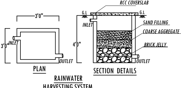
RAINWATER HARVESTING SYSTEM
