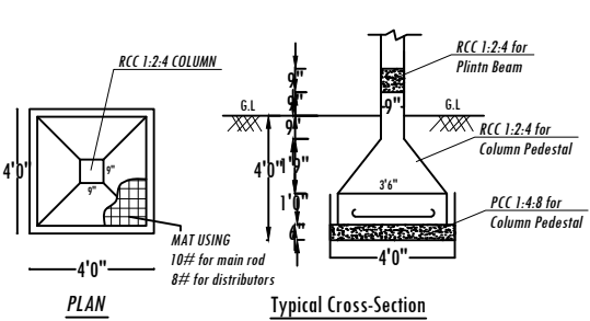
Typical Cross-Section
