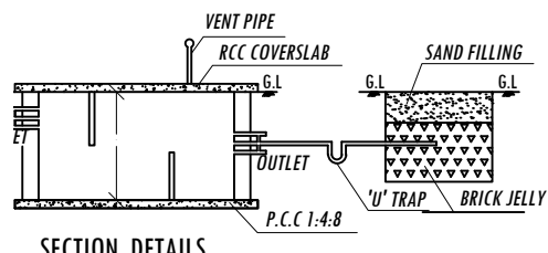
SEPTIC TANK AND DISPERSION TRENCH DETAILS
