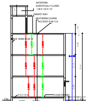
SECTION "A-B"
