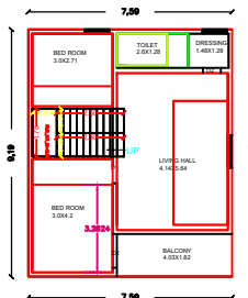
PRO. SECOND FLOOR PLAN.
