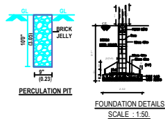
FOUNDATION DETAILS SCALE : 1:50
