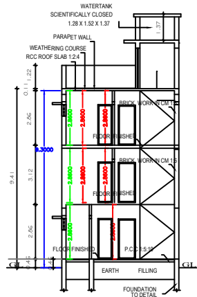
SECTION "A-B"
